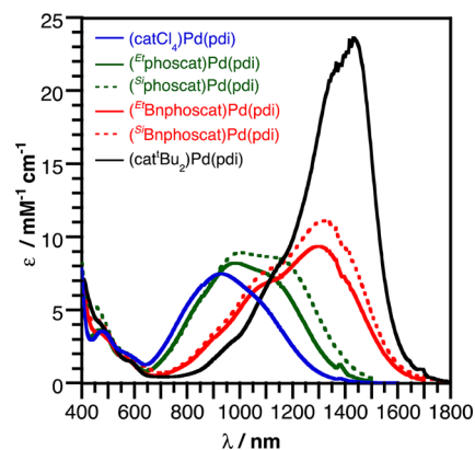
Figure 1. UV-vis-NIR absorption spectra of (catecholate)Pd(pdi) complexes in CH 2 Cl 2 at 298 K.
