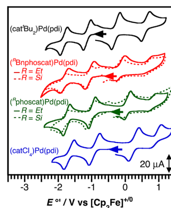
Figure 2. Cyclic voltammetry plots for (catecholate)Pd(pdi) complexes. Data acquired at 298 K on 1 mM samples dissolved in CH 2 Cl 2 containing 0.1 M [nBu 4 N][PF 6 ] using a glassy-carbon electrode and a scan rate of 200 mV s -1 . Potentials were referenced to [Cp 2 Fe] +0 using an internal standard.
